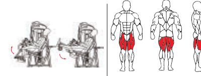
TB25 坐式伸屈腿训练器 SEATED LEG CURL/EXTENSION Weight:253kg Size:1480×990×1620mm Packing Size:1720×1120×520mm
