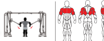
TF21 大飞鸟训练器 CABLE CROSSOVER Weight:339kg Size:3860×700×2330mm Packing Size:2690×1120×770mm
