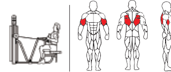
TB34 坐式划船训练器 VERTICAL ROW Weight:198kg Size:1570×1200×1620mm Packing Size:1720×1120×570mm
