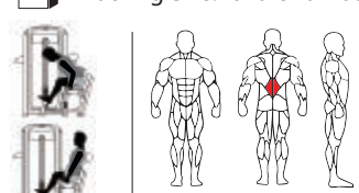
TE11 背肌训练器 BACK EXTENSION N.W:210kg size:1430×1170×1630mm Packing Size:1620×920×480mm
