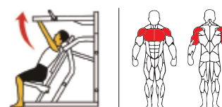
TM15 坐姿上斜推胸机 SEATED INCLINE CHEST PRESS Weight:130kg Size:1300×1690×1530mm Packing Size:1400×1120×520mm
