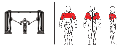
TB16 大飞鸟训练器 ADJUSTABLE CROSSOVER Weight:312kg Size:3860×715×2270mm Packing Size:2690×1120×740mm
