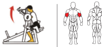
TM29 坐式二头肌训练机 SEATED BICEPS Weight:98kg Size:1510×1460×1470mm Packing Size:1420×1120×470mm
