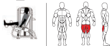
TF14 坐式曲腿训练器 SEATED LEG CURL Weight:276kg Size:1660×1280×1630mm Packing Size:1620×1120×480mm
