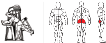
TB24 后抬腿训练器 GLUTE ISOLATOR Weight:189kg Size:1190×900×1620mm Packing Size:1720×1120×570mm
