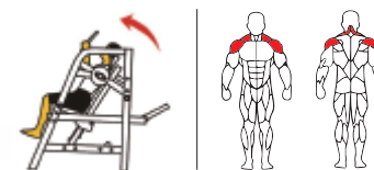
TM68 臂下压背肌训练器 PULL OVER Weight: 160kg Size: 1680×1920×1830mm Packing Size: 1580×1320×520mm
