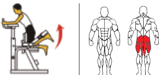
TM66 屈腿训练器 KNEELING LEG CURL Weight: 110kg Size: 1170×1800×1410mm Packing Size: 1270×1470×500mm
