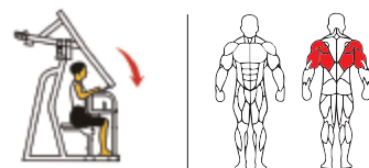
TM02 划艇高拉背训练器 HIGH ROW Weight:159kg Size:1610×1530×2010mm Packing Size:1670×1120×520mm
