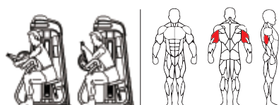
TB28 45度三头肌训练器 TRICEPS EXTENSION Weight:177kg Size:1290×960×1620mm Packing Size: 1720×1120×400mm
