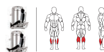
TF17 坐式小腿训练器 SEATED CALF TRAINER Weight:230kg Size:1340×1120×1630mm Packing Size:1620×920×400mm
