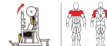
TM10 举重架 VERTICAL BENCH Weight:100kg Size:1840×1250×1660mm Packing Size:1720×1120×420mm
