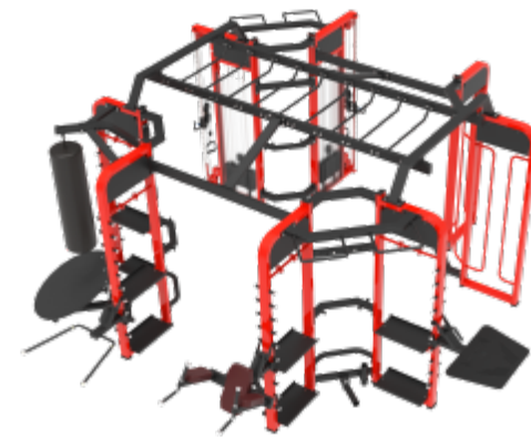
360A SYNERGY 360(8 GATES) Weight:1520kg Size:4430×4430×2560mm Packing Size:(2370×3)×1120×820mm
