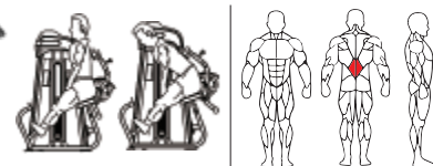
TB31 背肌训练器 BACK EXTENSION Weight:182kg Size:1255×990×1620mm Packing Size: 1720×1120×620mm
