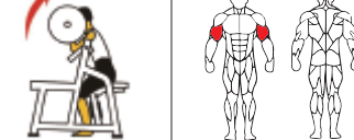
TN20 肱二头肌训练机 ARM CURL Weight:79kg Size:1150×820×1060mm Packing Size:1200×1140×420mm
